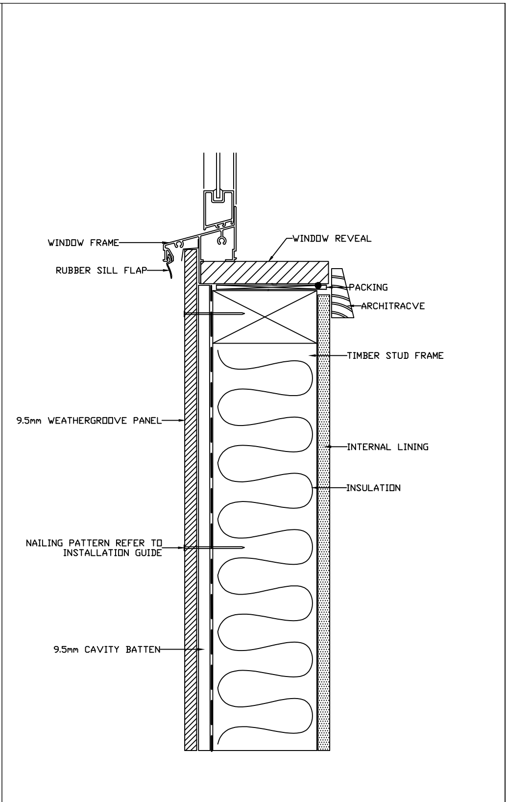
WINDOW SILL DETAIL
