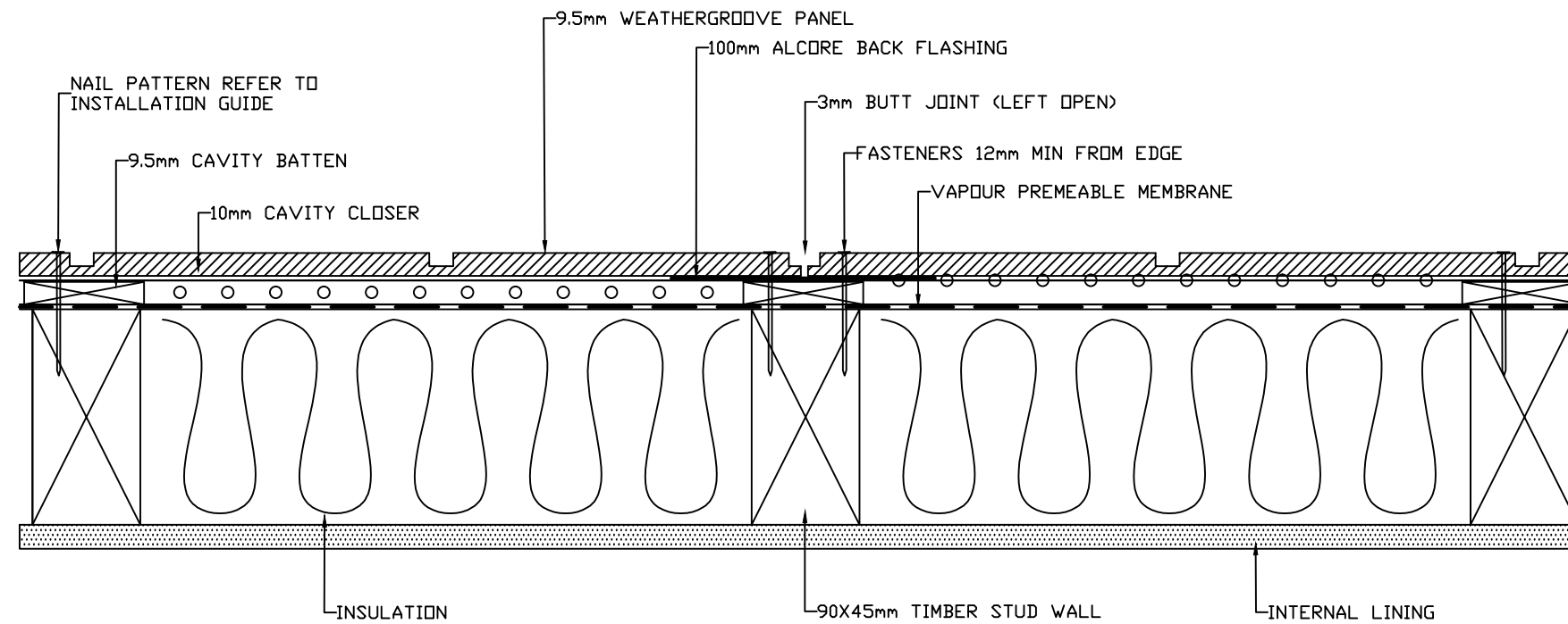
ON STUD BUTT JOIN DETAIL
