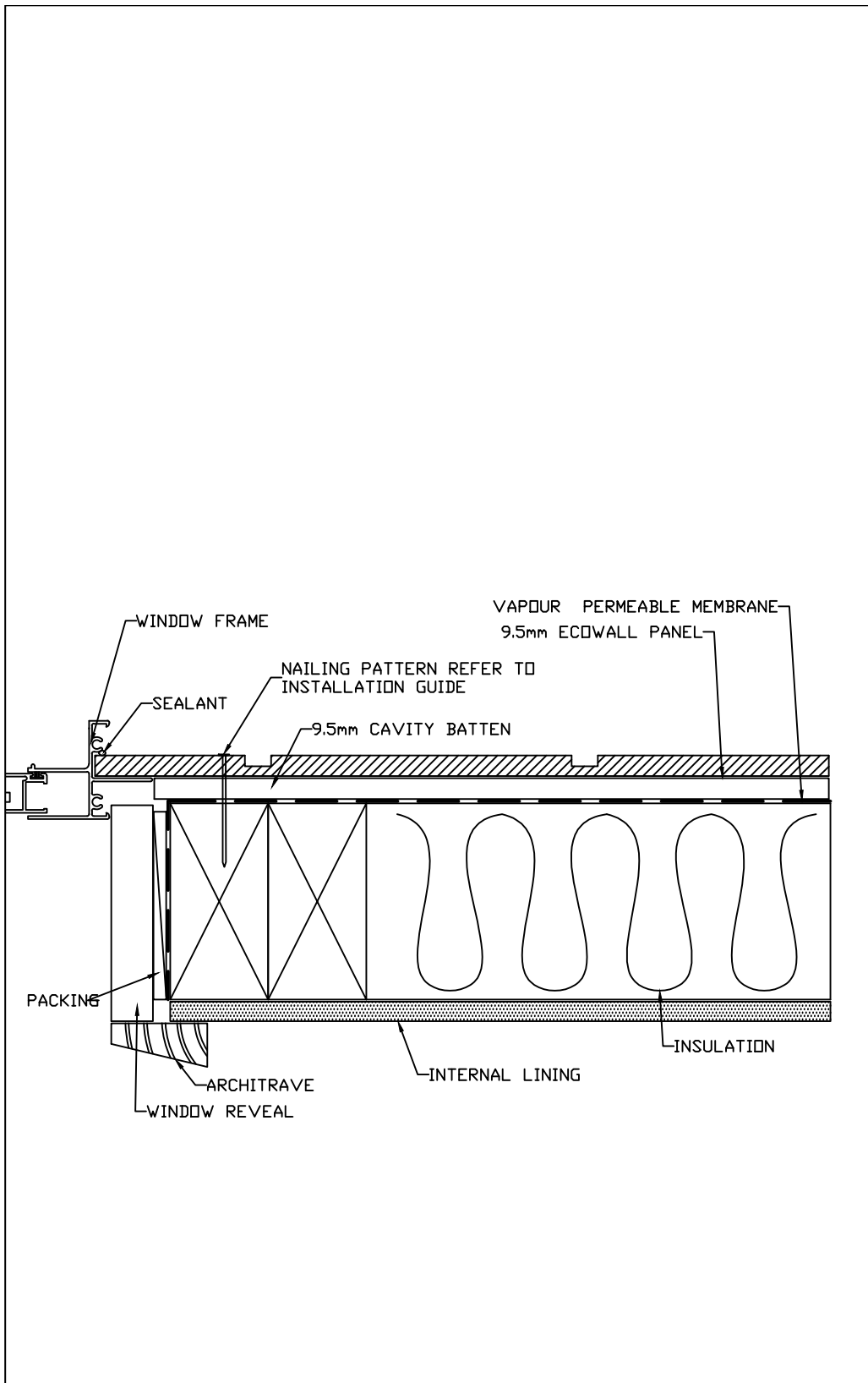
WINDOW JAMB DETAIL
