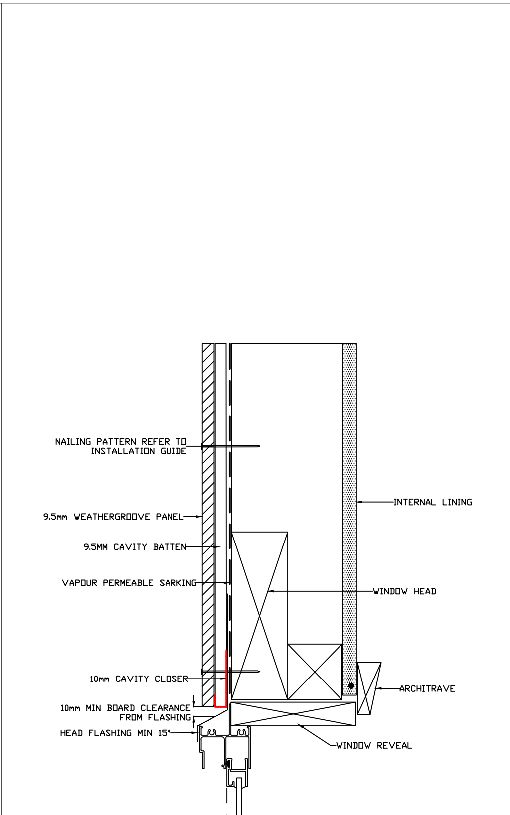
WINDOW HEAD DETAIL
