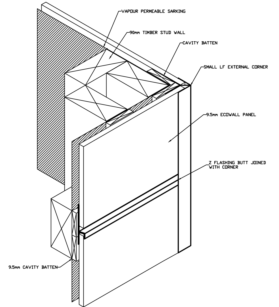
Z FLASHING INTO CORNER DETAIL
