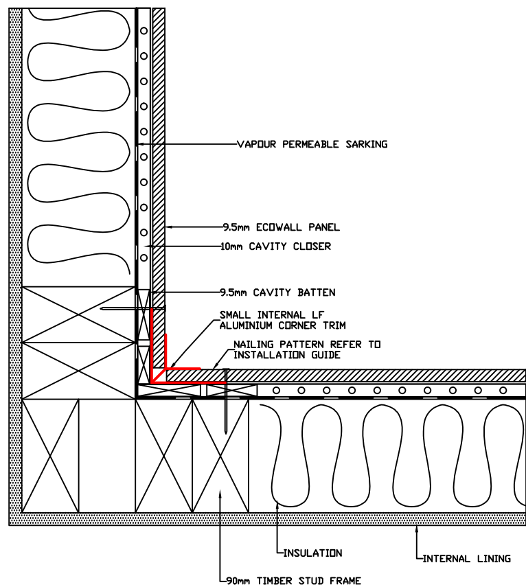
SMALL INTERNAL LF CORNER DETAIL
