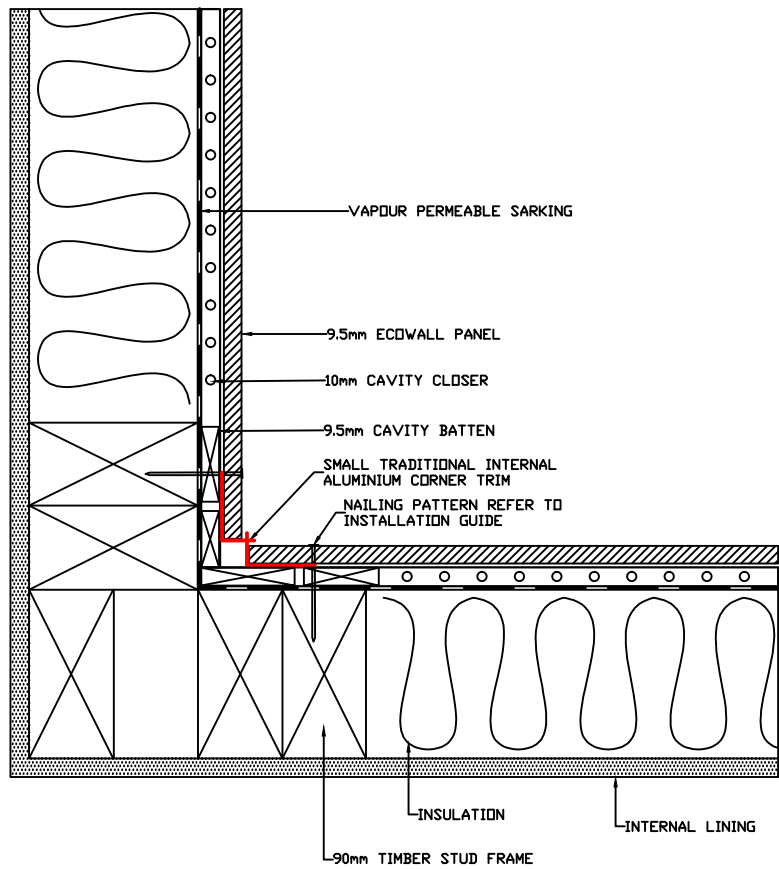
SMALL TRADITIONAL INTERNAL "W" CORNER DETAIL
