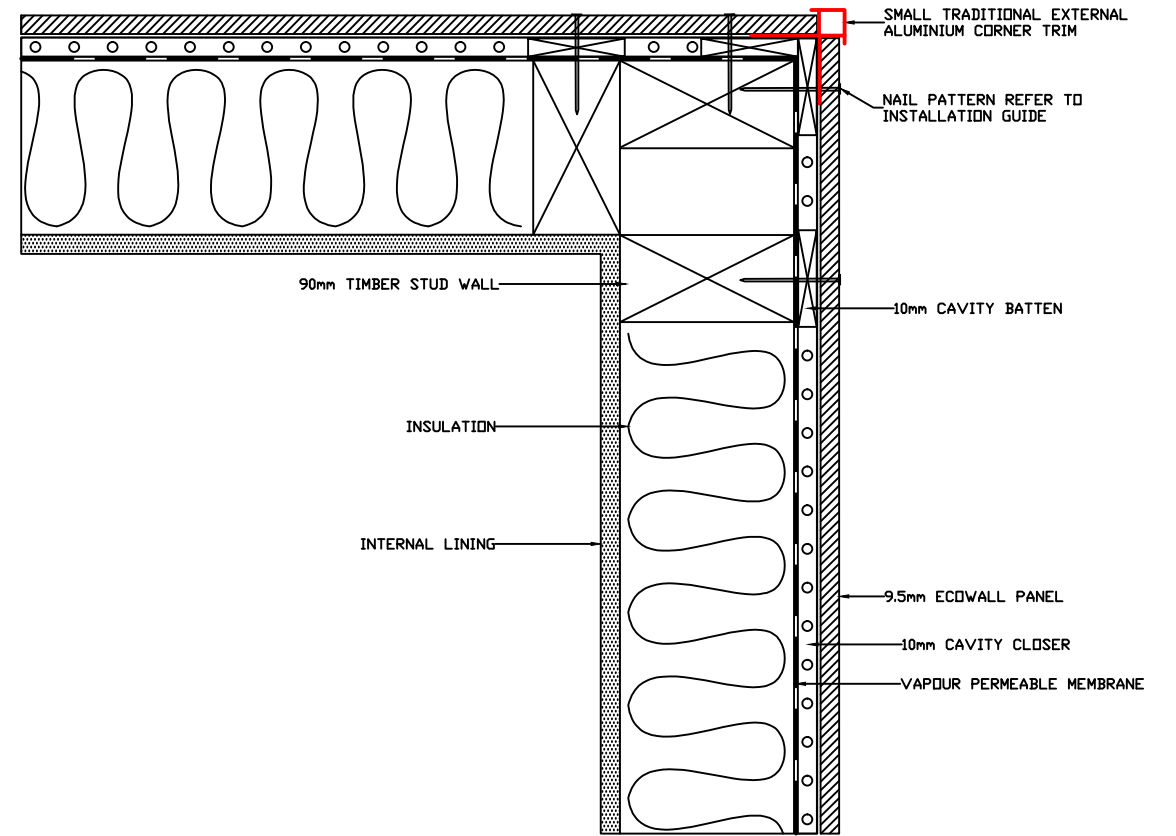
SMALL TRADITIONAL EXTERNAL "BOX" CORNER DETAIL
