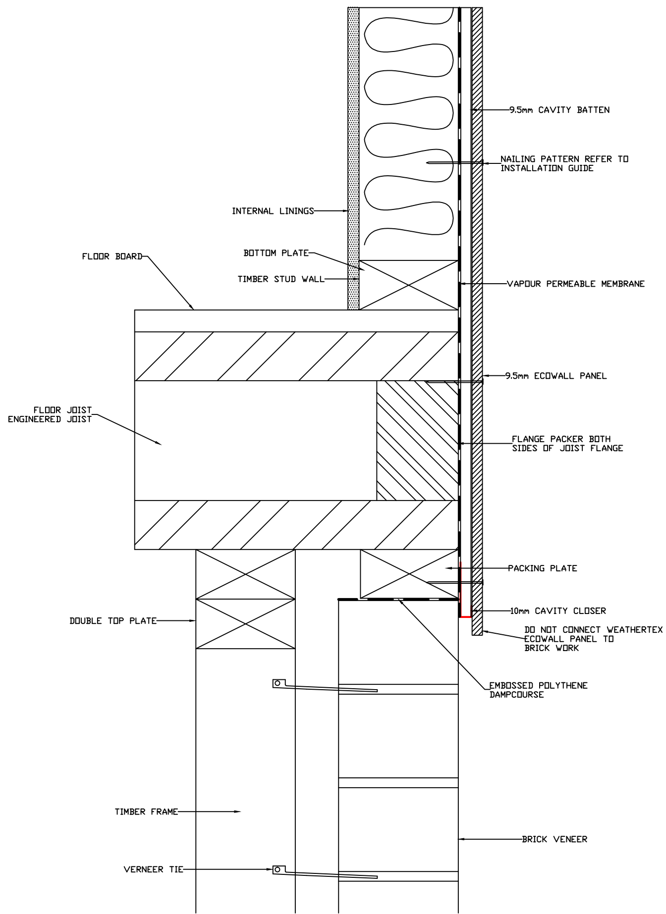
FLUSH WITH BRICK VENEER DETAIL
