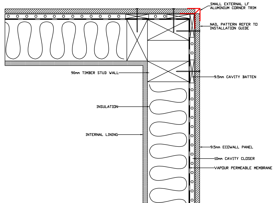
SMALL EXTERNAL LF CORNER DETAIL
