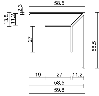
Small Internal LF Aluminium Corner
