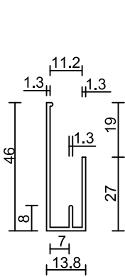
Small Window Surround LF Aluminium
