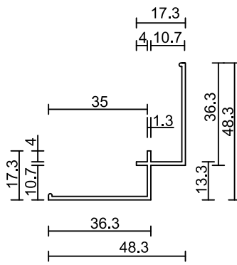
Small Internal Aluminium Corner
