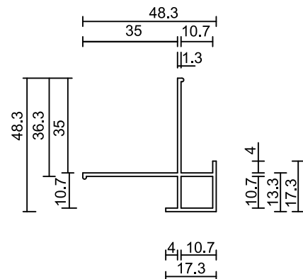
Small External Aluminium Corner
