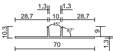
Aluminium Deep Channel Joiner
