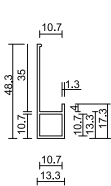
Small End Stop Aluminium
