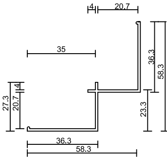
Large Internal Aluminium Corner
