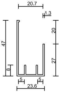
Large Window Surround LF Aluminium
