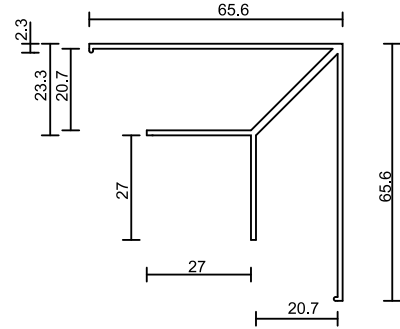
Large Internal LF Aluminium Corner
