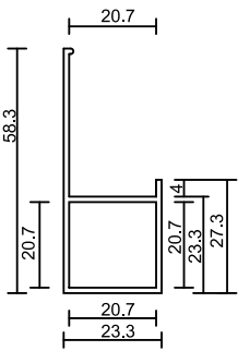
large End Stop Aluminium
