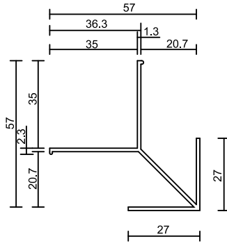
Large External LF Aluminium Corner
