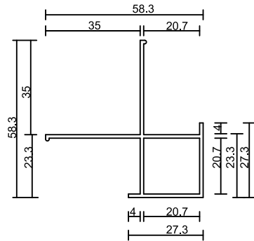
Large External Aluminium Corner
