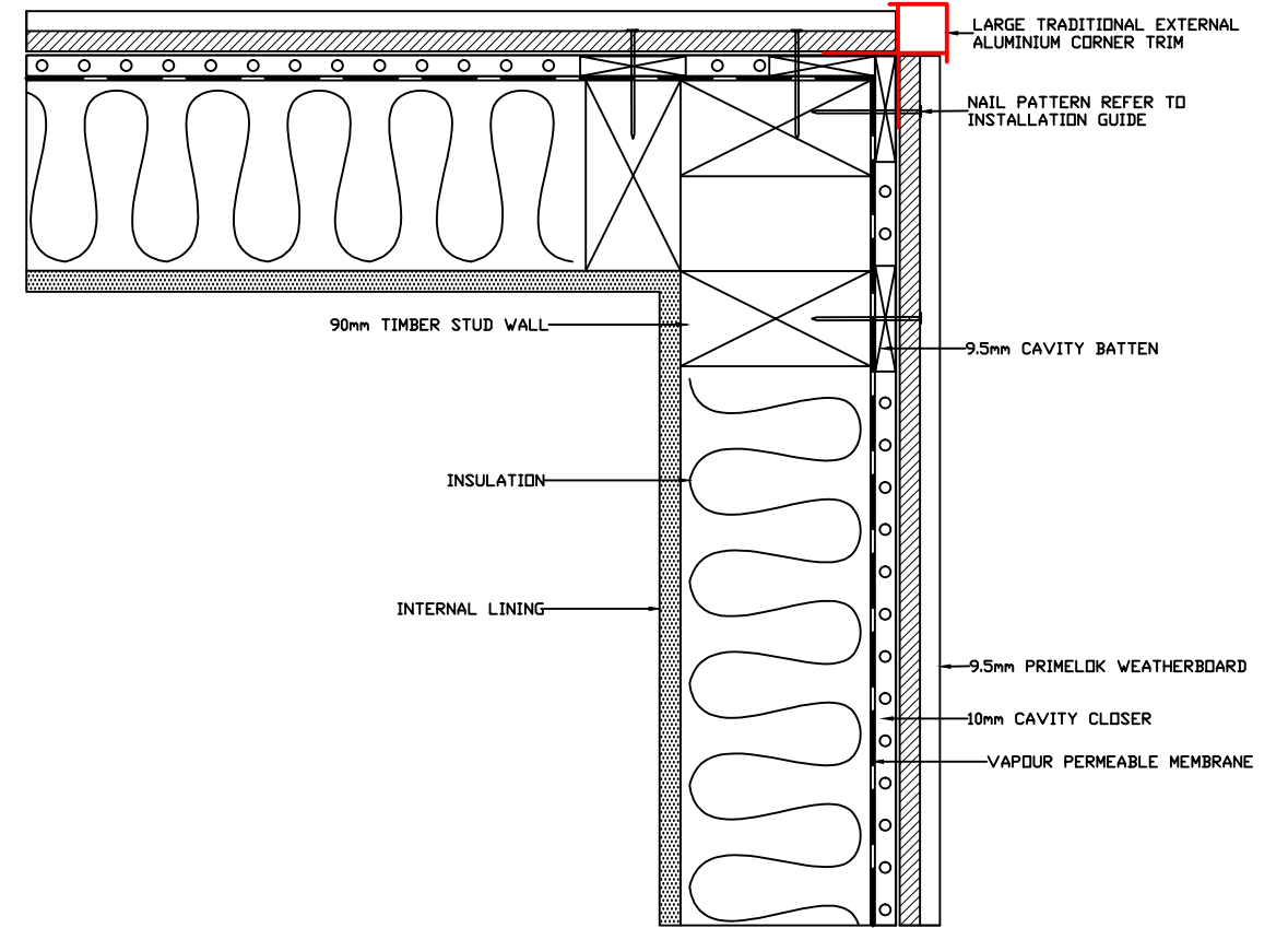
LARGE TRADITIONAL EXTERNAL "BOX" CORNER DETAIL
