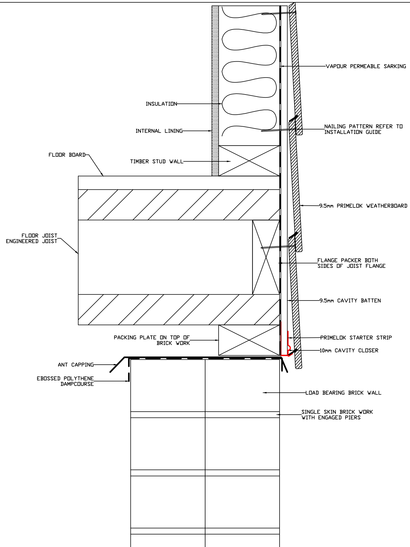
OVER DOUBLE BRICK PIER DETAIL
