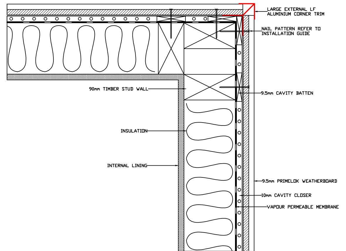
LARGE EXTERNAL LF CORNER DETAIL
