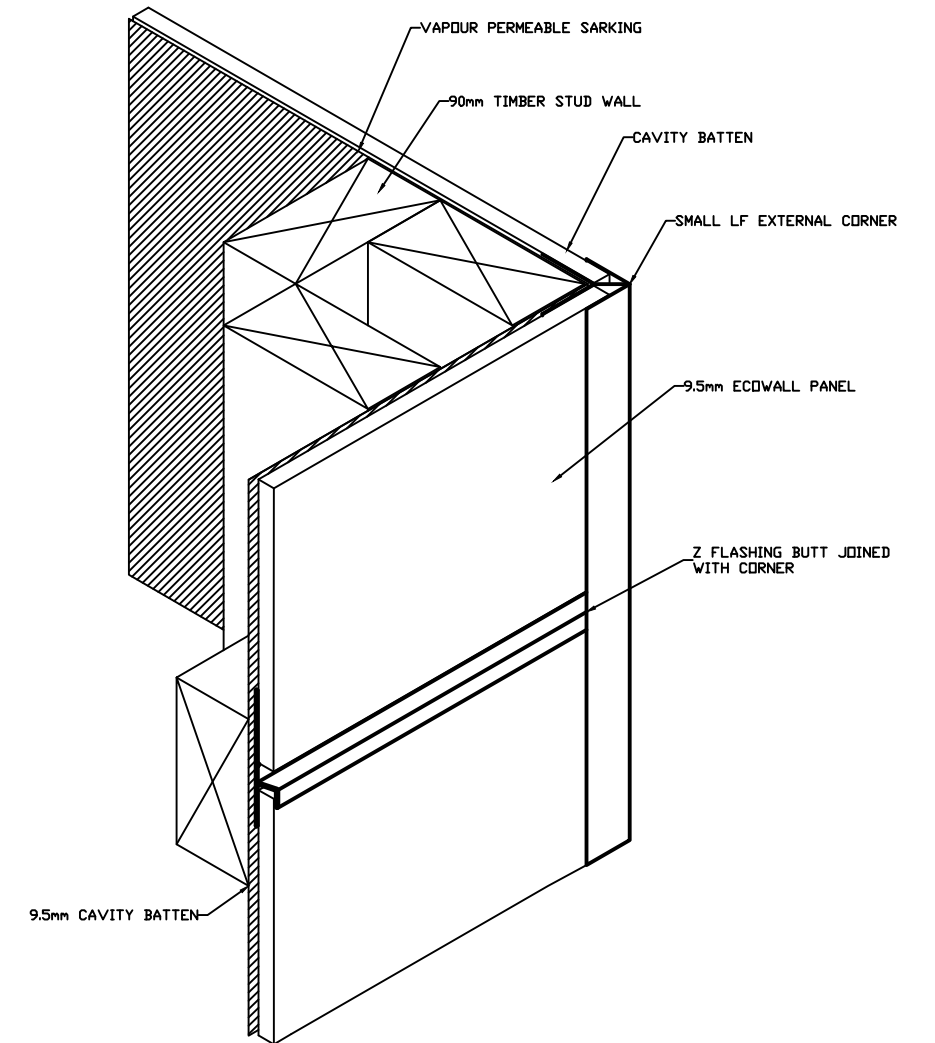
Z FLASHING INTO CORNER DETAIL
