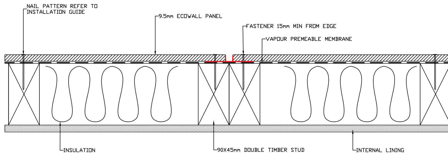
DEEP CHANNEL JOINDER DETAIL
