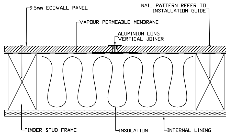
LONG VERTICAL JOINDER DETAIL
